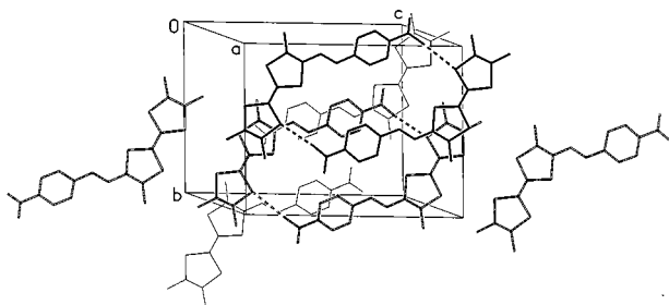
Figure 5. Crystal packing of 9 , projection on the (1 0 -1) plane
